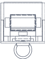
DETAIL A: END VIEW Scale 1:5; from the handle end
