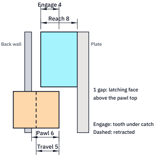
DETAIL B: CATCH GEOMETRY
