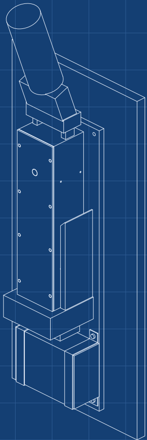
ISOMETRIC VIEW
