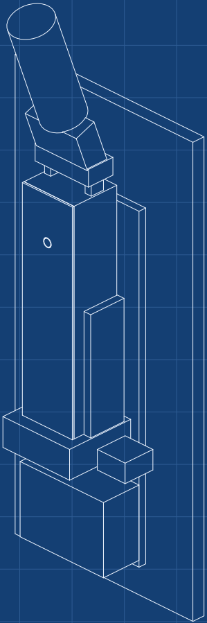
ISOMETRIC VIEW Not to scale; grey is for scale; seen from the front right and above, about 30 deg elevation
