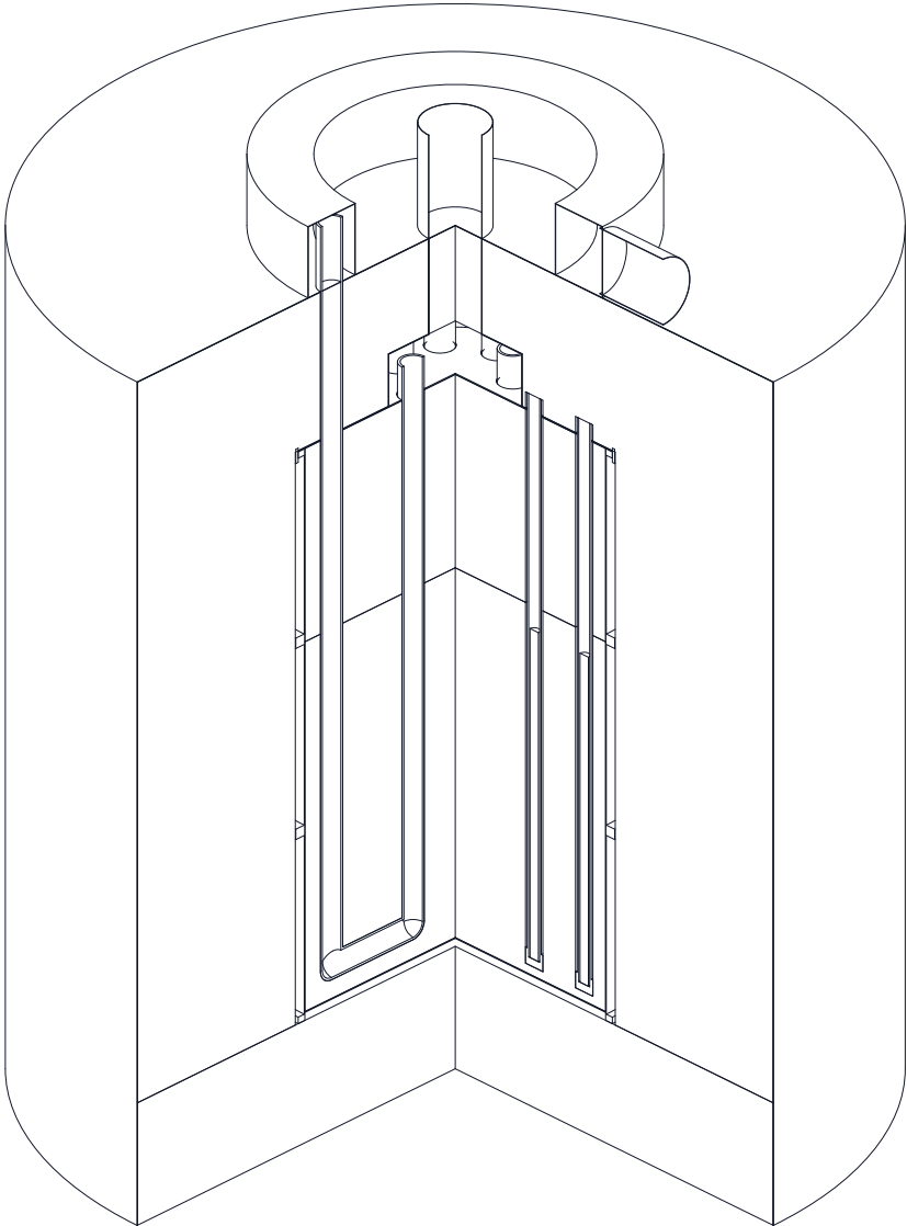
ISOMETRIC CUTAWAY Quarter removed, not to scale
