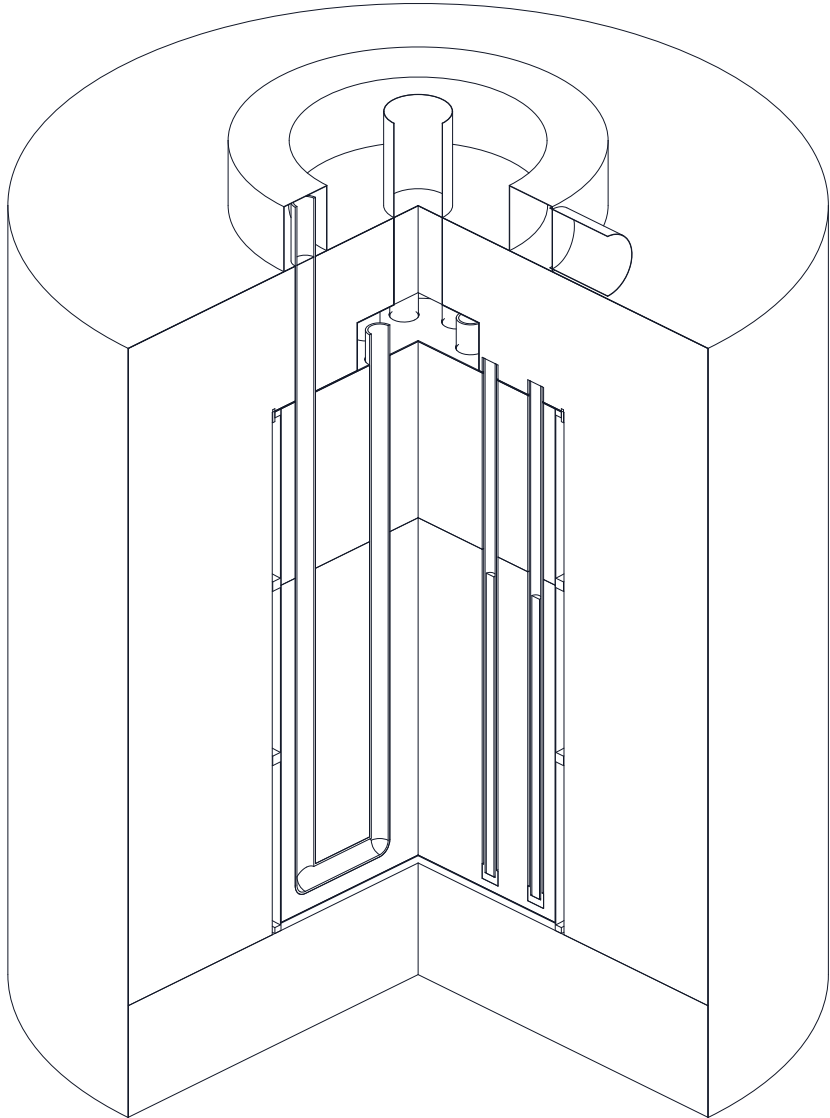
ISOMETRIC CUTAWAY Quarter removed, not to scale
