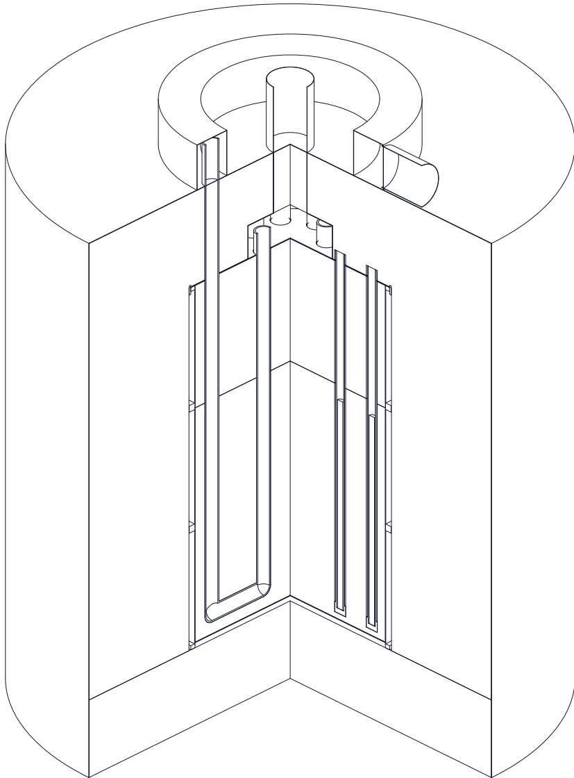
ISOMETRIC CUTAWAY
