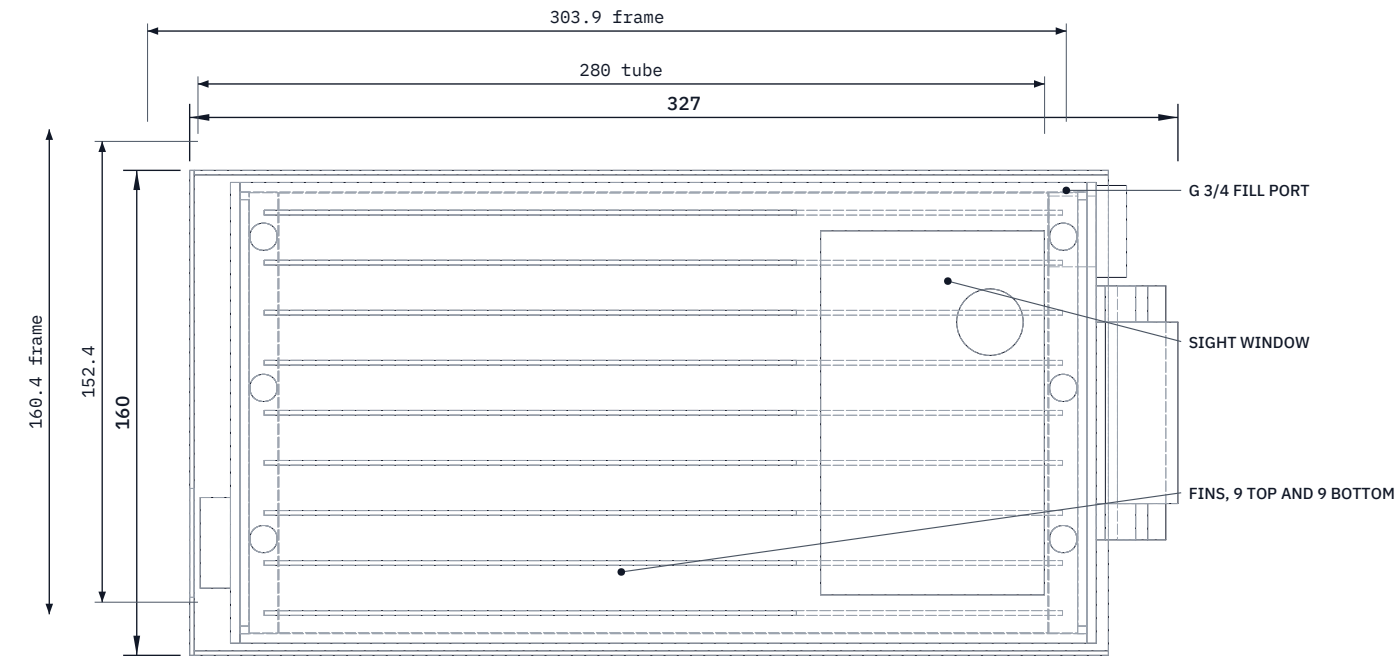
TOP VIEW
