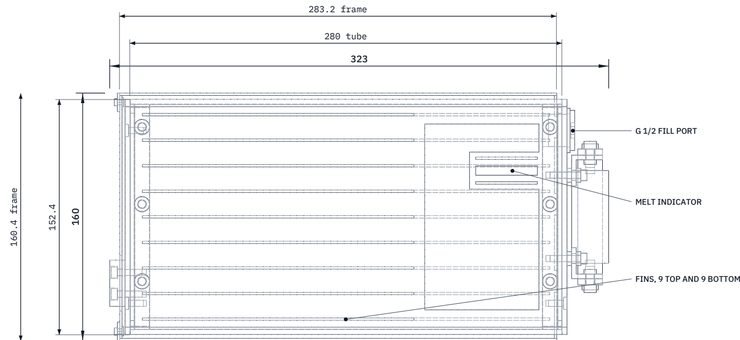
TOP VIEW
