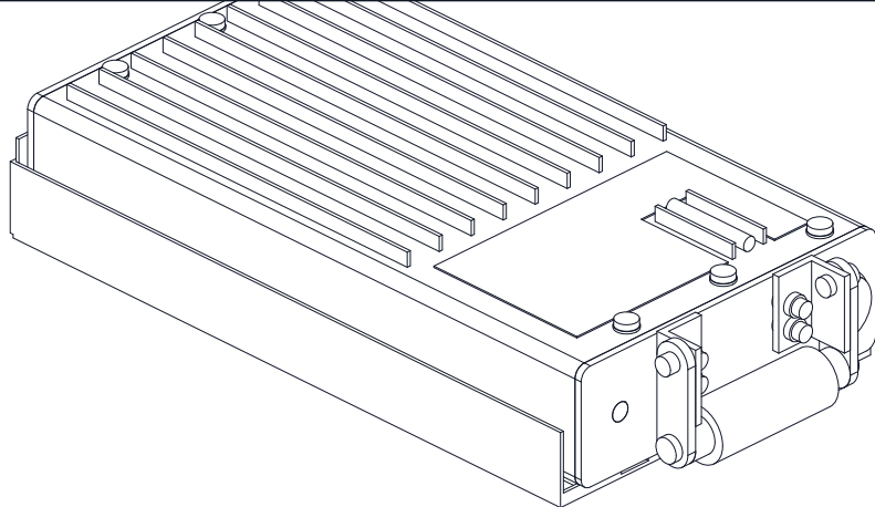
ISOMETRIC VIEW
