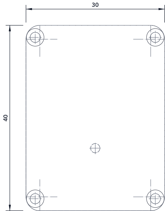
TOP VIEW Scale 2:1; looking down (along -Z)
