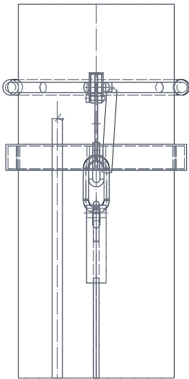
RIGHT VIEW
