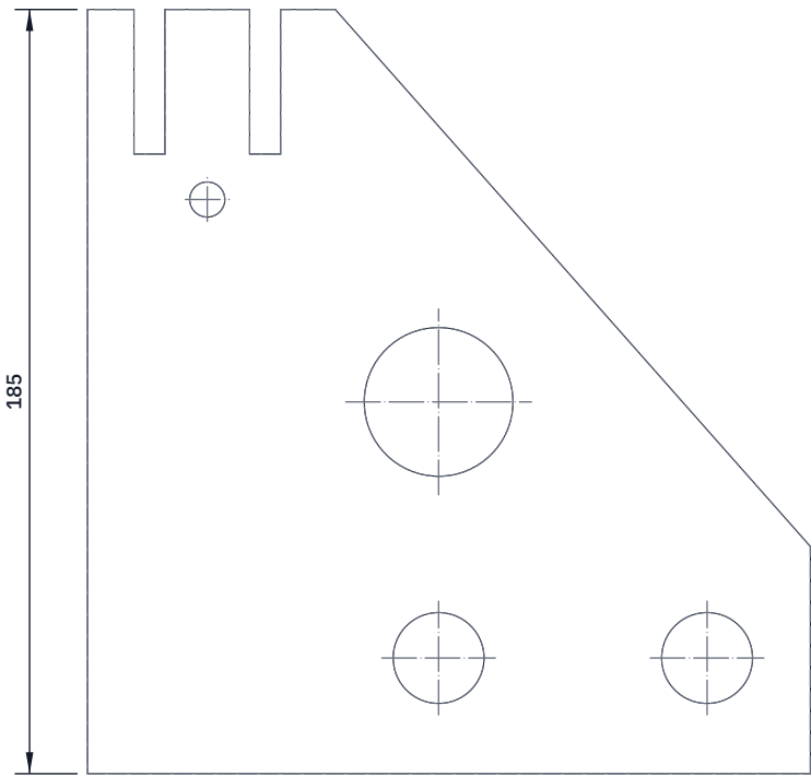
FRONT VIEW Scale 1:2; looking at the front (along +Y)
