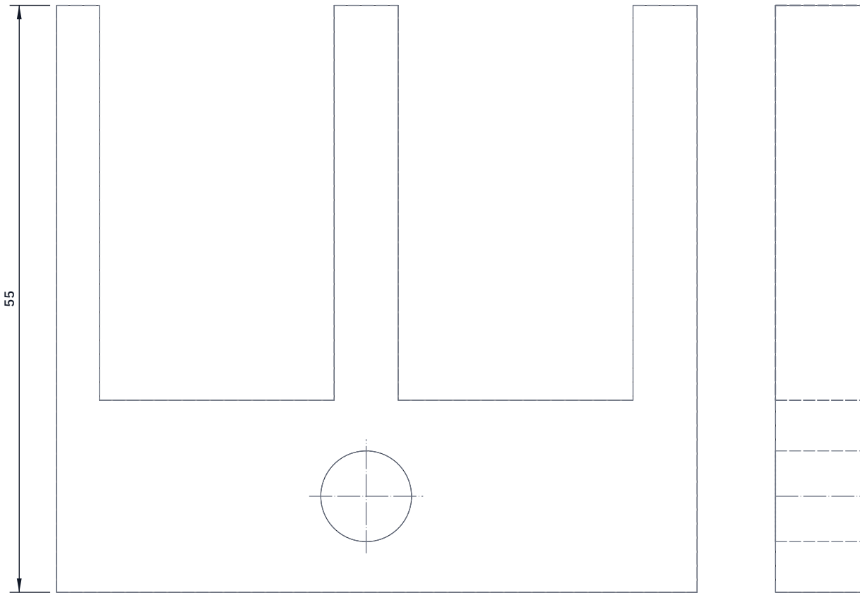
FRONT VIEW Scale 2:1; looking at the front (along +Y)
