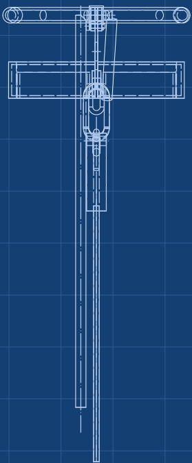
RIGHT VIEW Scale 1:10; looking at the right side (along -X)
