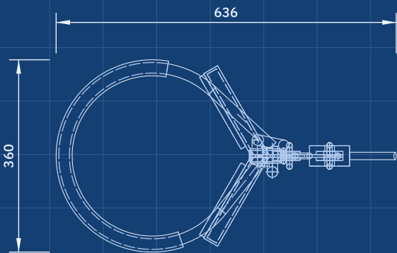
TOP VIEW Scale 1:10; looking down (along -Z)
