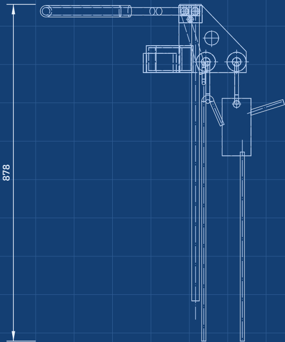
FRONT VIEW Scale 1:10; looking at the front (along +Y)
