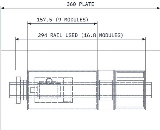
TOP VIEW Scale 1:5
