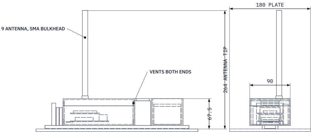
FRONT VIEW Scale 1:5
