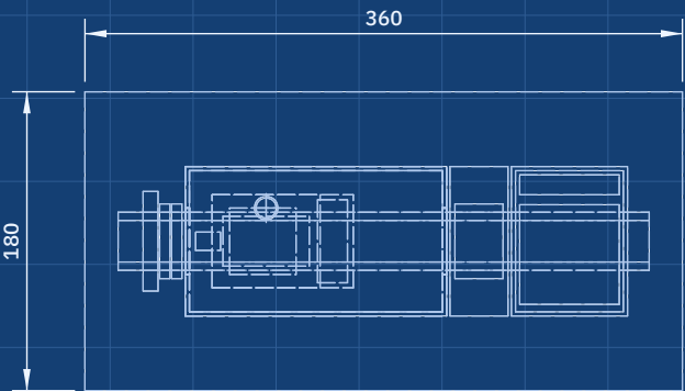
TOP VIEW Scale 1:5; looking down (along -Z)
