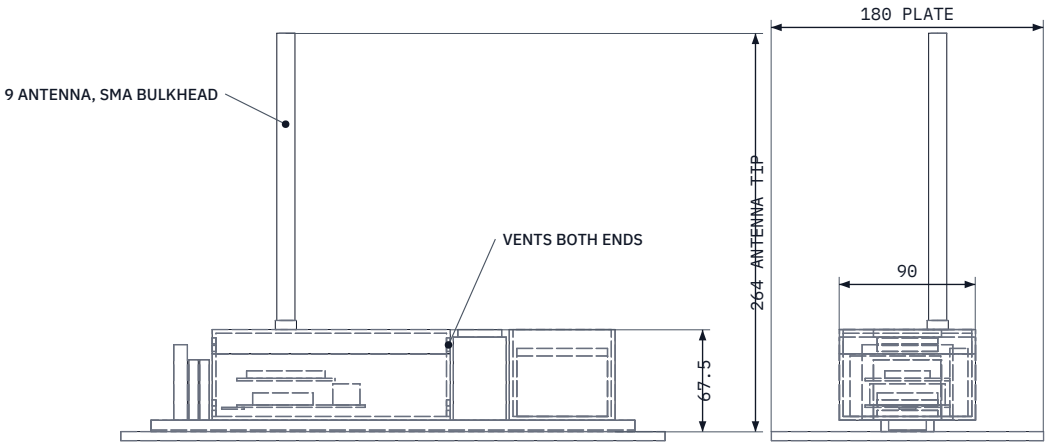
FRONT VIEW Scale 1:5
