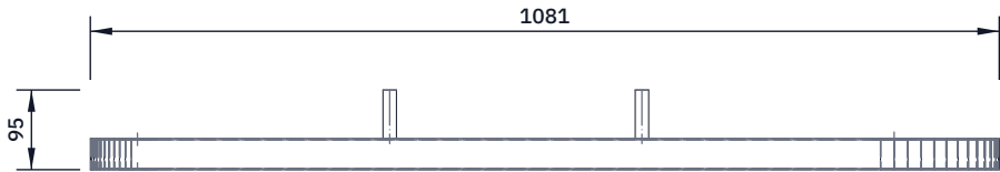
TOP VIEW Scale 1:10; looking down (along -Z)
