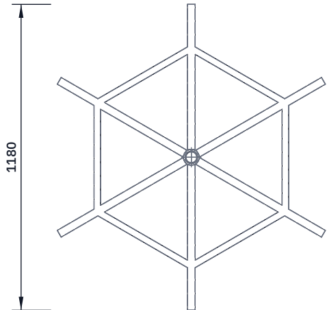
FRONT VIEW Scale 1:20; looking at the front (along +Y)
