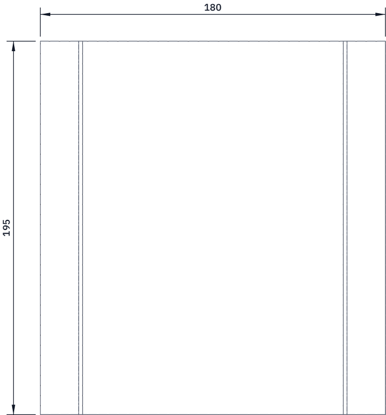
TOP VIEW Scale 1:2; looking down (along -Z)
