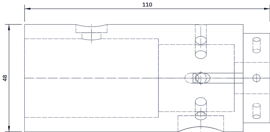
TOP VIEW Scale 1:1; looking down (along -Z)
