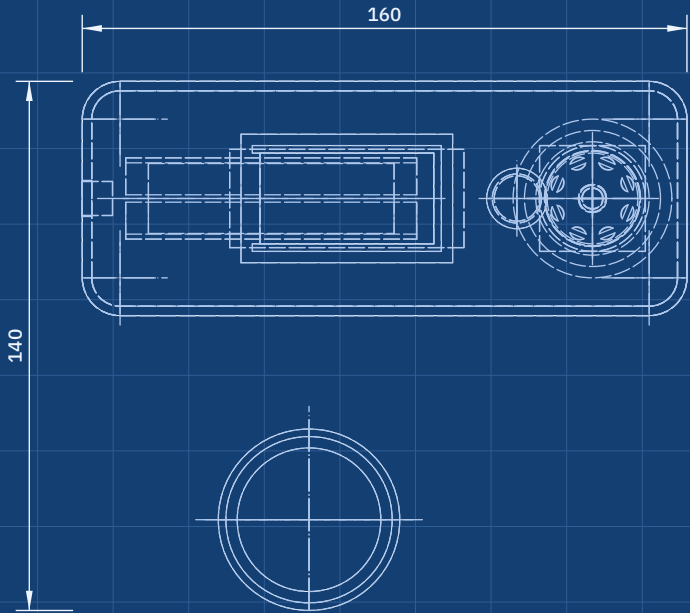
TOP VIEW Scale 1:2; looking down (along -Z)
