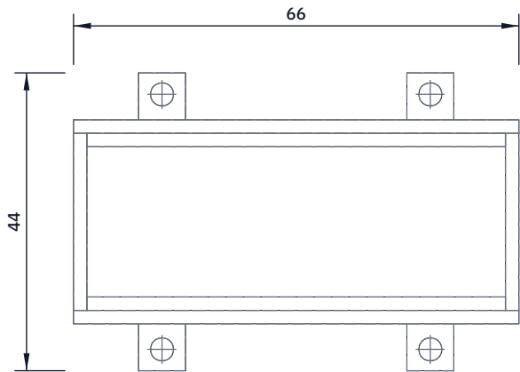
TOP VIEW Scale 1:1; looking down (along -Z)
