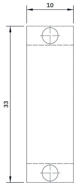
TOP VIEW
