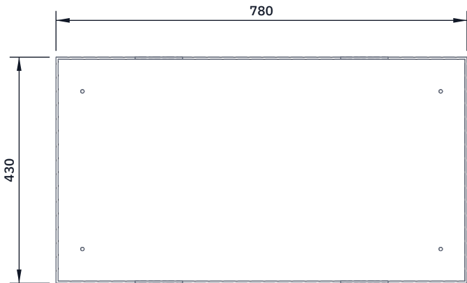
TOP VIEW Scale 1:10; looking down (along -Z)
