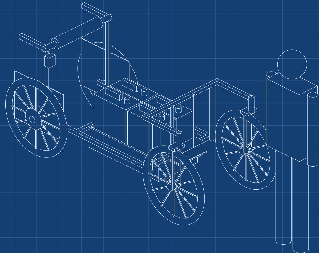
ISOMETRIC VIEW Not to scale; figure is a 1.75 m person
