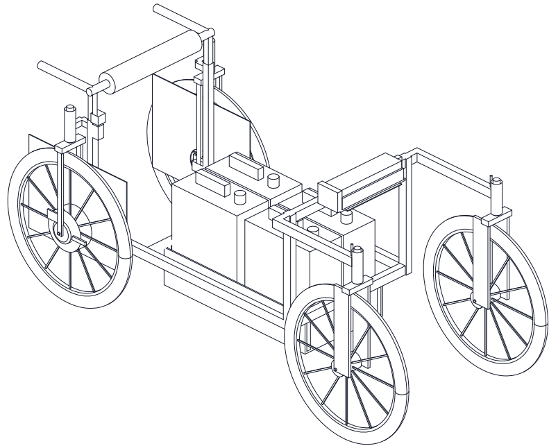
ISOMETRIC VIEW Not to scale; assist kit shown fitted
