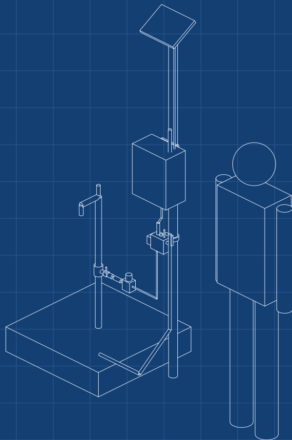
ISOMETRIC VIEW
