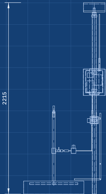
FRONT VIEW
