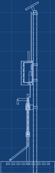
RIGHT VIEW Scale 1:25
