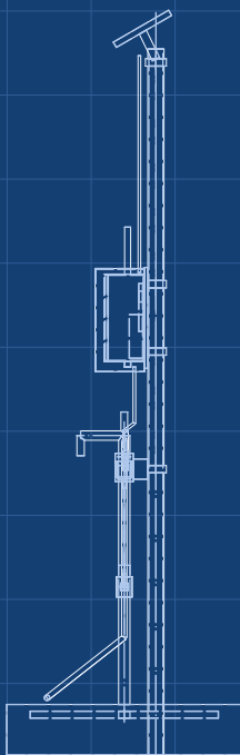
RIGHT VIEW
