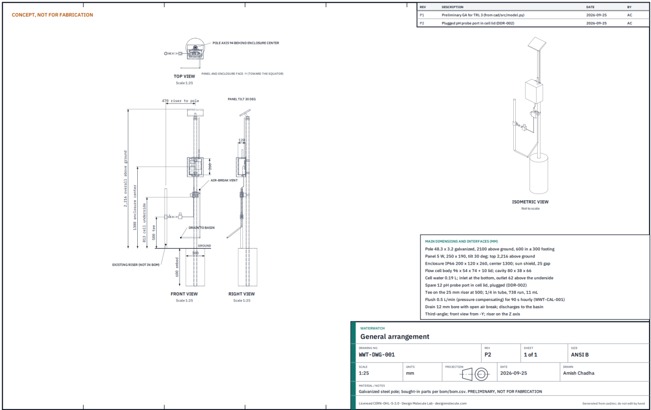
Figure 4. General arrangement WWT-DWG-001, Rev P2, generated from cad/src/model.py by cad/src/sheets.py . Preliminary, not for fabrication.
