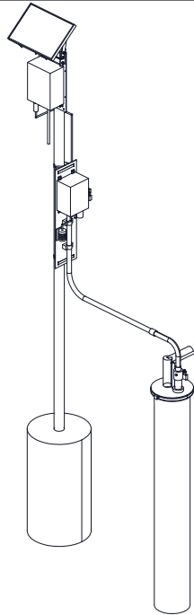
ISOMETRIC VIEW
