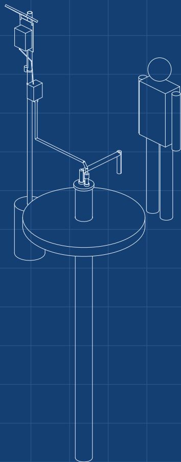
ISOMETRIC VIEW
