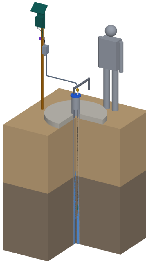
Figure 1. Concept massing model in a borehole with a pump and riser, soil cut open, 1.75 m person for scale. The borehole is shortened for display. CONCEPT, NOT FOR FABRICATION.
