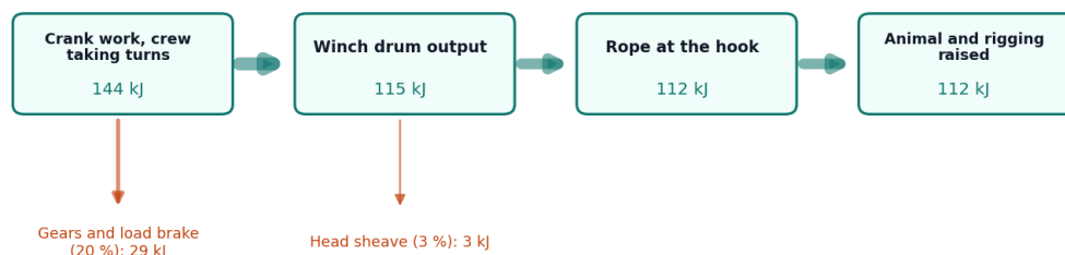
Figure 3. Energy to lift the design animal from 15 m down to the landing height (estimates).
