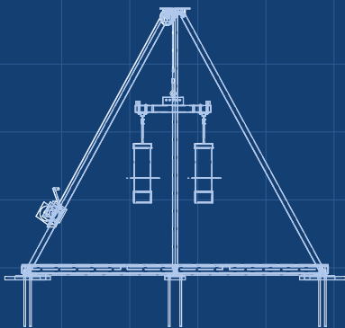
RIGHT VIEW
