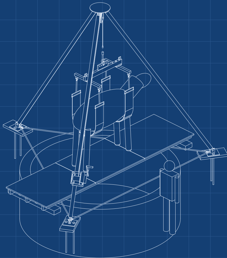
ISOMETRIC VIEW
