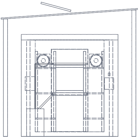
RIGHT VIEW Scale 1:50
