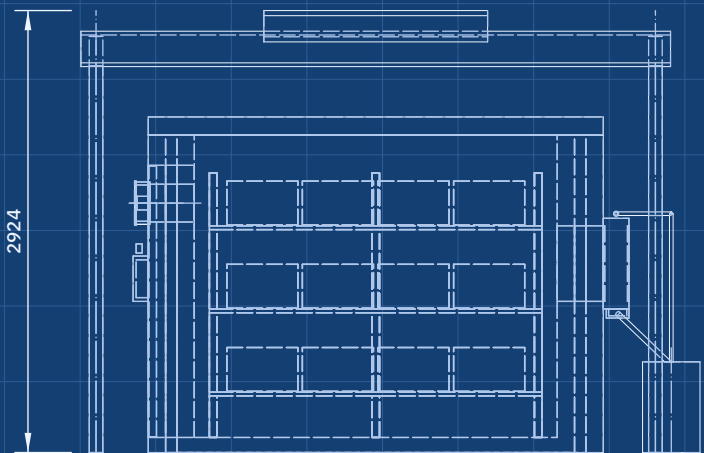
FRONT VIEW Scale 1:50; looking at the front (along +Y)
