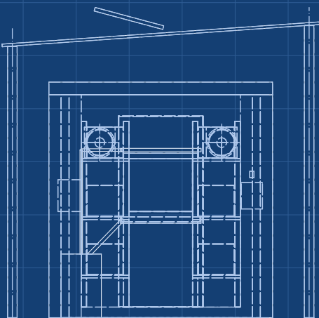
RIGHT VIEW Scale 1:50; looking at the right side (along -X)
