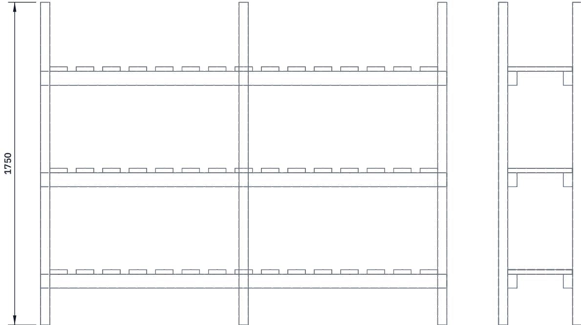
FRONT VIEW Scale 1:20; looking at the front (along +Y)
