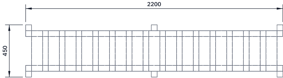
TOP VIEW Scale 1:20; looking down (along -Z)
