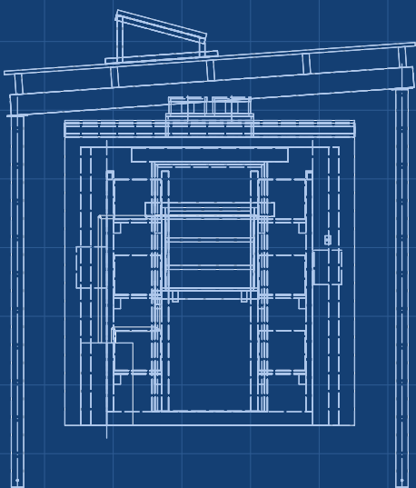
RIGHT VIEW
