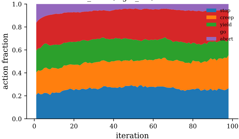
2_dense/right_left/DRPPO
