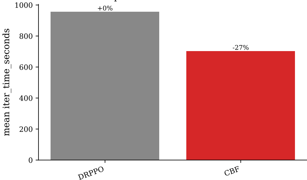
Computational overhead vs DRPPO
