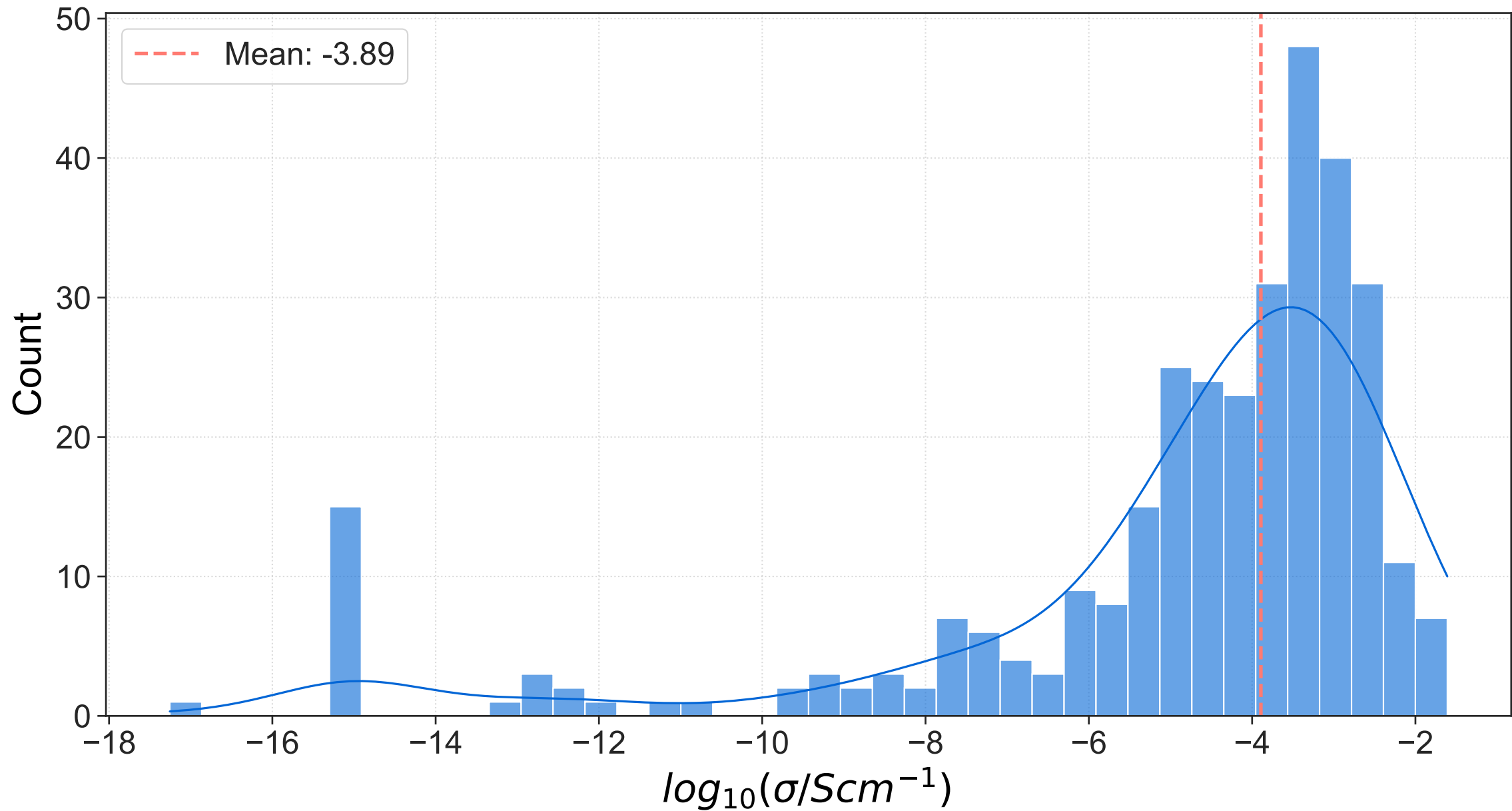
Distribution of Ionic Conductivities (RT / 25 °C)
