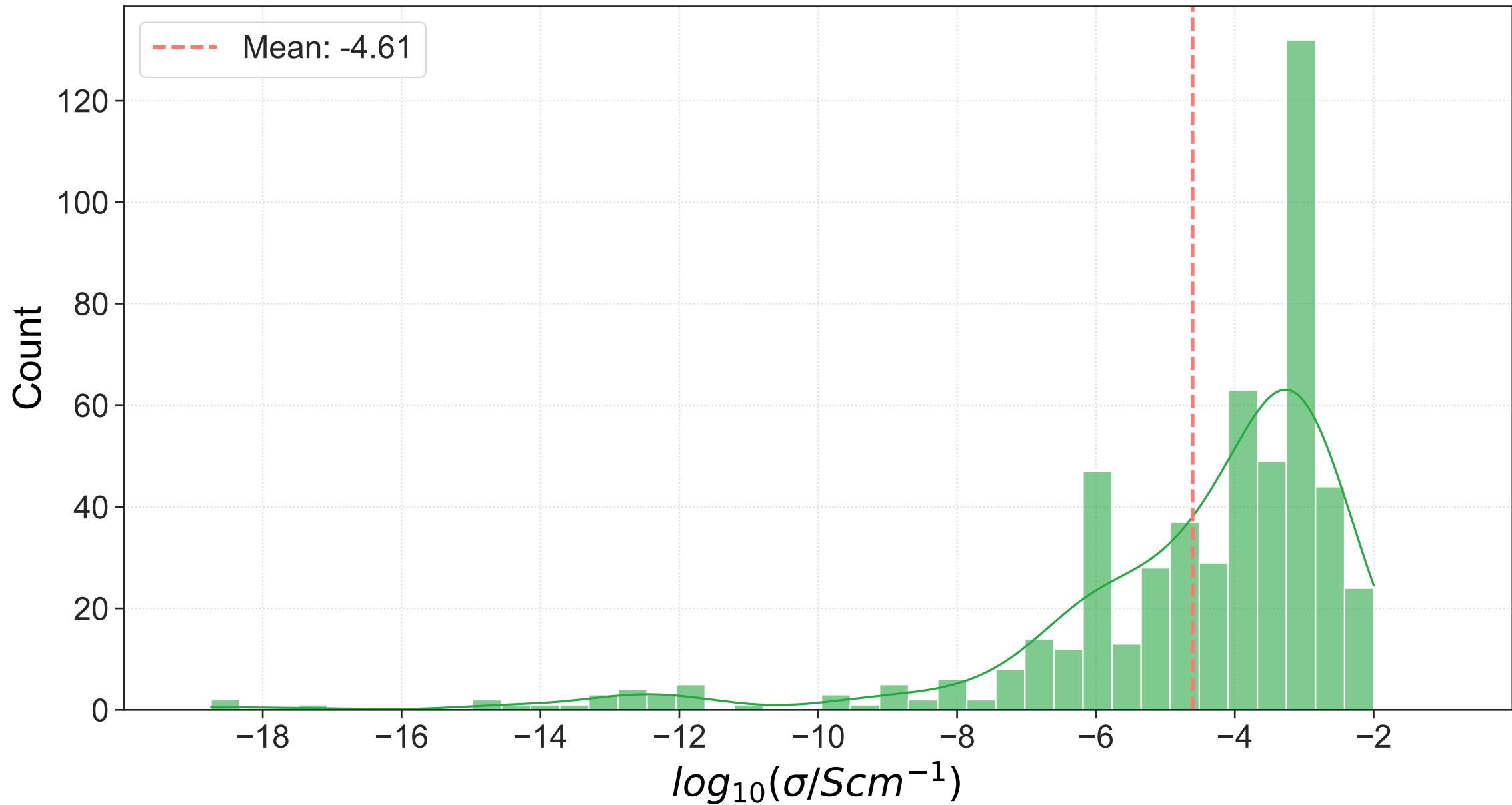
Distribution of Extracted Ionic Conductivities (RT)
