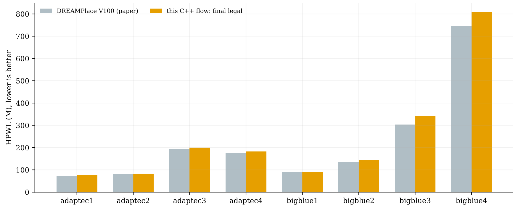
Final legal HPWL versus DREAMPlace Table II V100 reference
