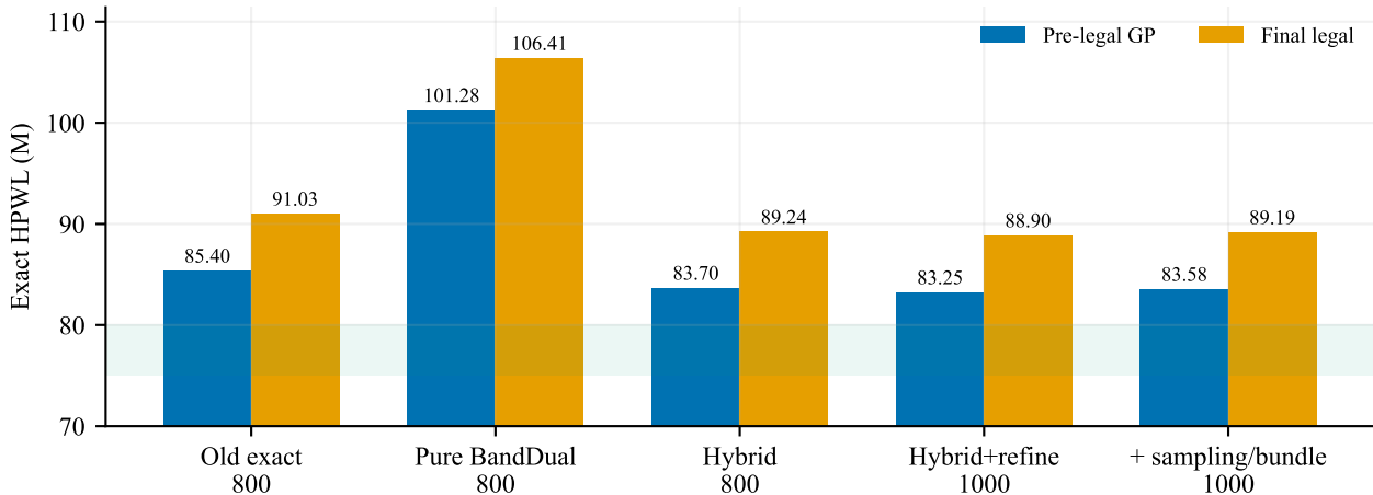
Ablation of density control and feasible-band refinement
