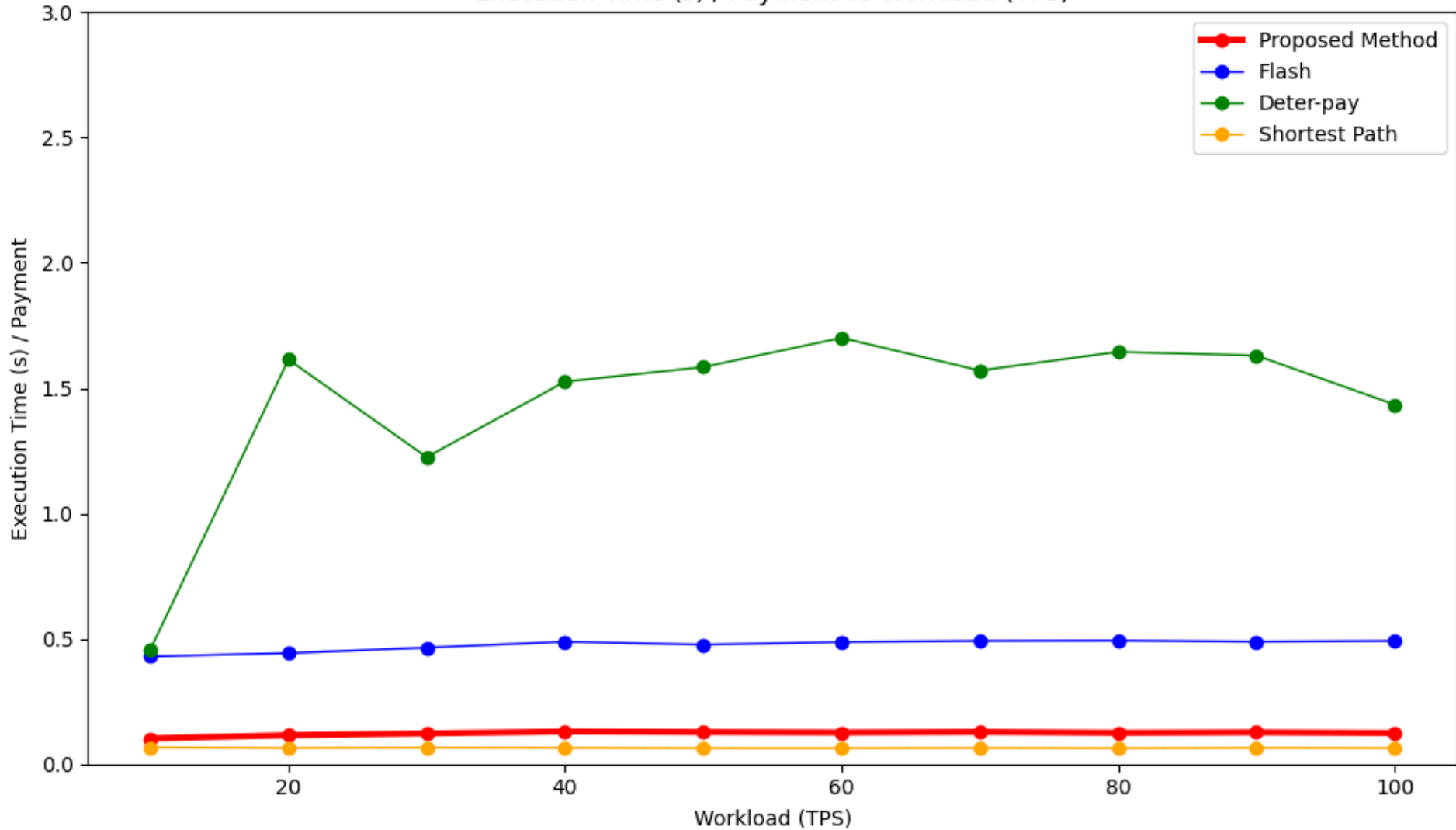
Execution Time (s) / Payment vs Workload (TPS)
