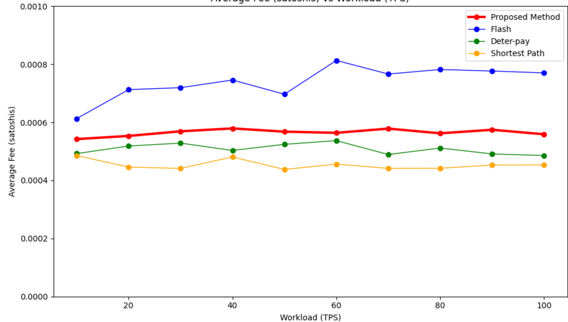
Average Fee (satoshis) vs Workload (TPS)
