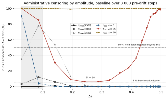
Figure 11. Censoring at H = 2000 of every censorable duration, by amplitude, one series per duration, with the 50% line above which no median is reported and the 5% line of the benchmark criterion. What to see: \tau_{\text{swap}}(75\%) peaks at 78% at \Delta e = 0.085 and is still above 50% at \Delta e = 0.141 , the lowest amplitude of the decision domain, but only 35% at the very bottom of the grid, and it falls under 5% from \Delta e = 0.243 ; \tau_{\text{det}} at \lambda = 25 is U-shaped, below 10% only between \Delta e = 0.19 and 0.33 ; at \lambda = 50 it never leaves 99%. Tables QCD_correlations_stratifiedes_full and QCD_socle_deux_fenêtres.
