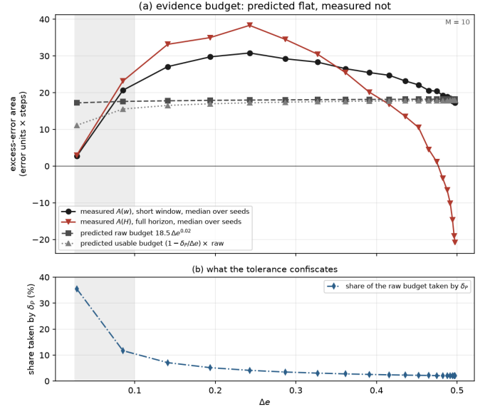
Figure 2. (a) Predicted budgets, raw 18.5 \Delta e^{0.02} and usable, against the measured areas A(w) and A(H) , medians over 100 seeds. (b) Share of the raw budget taken by the tolerance \delta_P . Shaded: the two amplitudes outside the decision domain of Question D.
