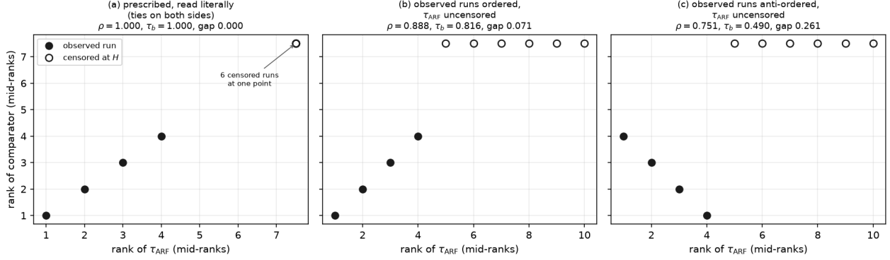
Figure 8. The three configurations of Table VII, as mid-ranks. Filled markers: observed runs; hollow markers: runs censored at H , which share one mid-rank on the comparator side. (a) The prescribed exercise read literally also ties the six censored runs on the \tau_{\text{ARF}} side, and the two coefficients coincide. (b) With \tau_{\text{ARF}} left uncensored, the same four ordered observations already separate Spearman from Kendall by 0.071. (c) Anti-ordering the four observations widens the gap to 0.261. Table QCD_contre_exemple_kendall .
