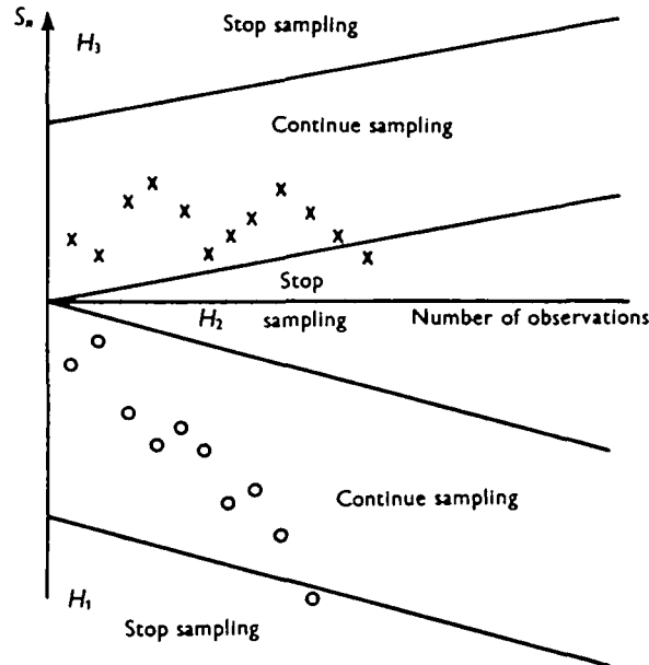
Fig. 2. A two-sided sequential test. O O sample path ending in H_1 . x x sample path ending in H_2 .
